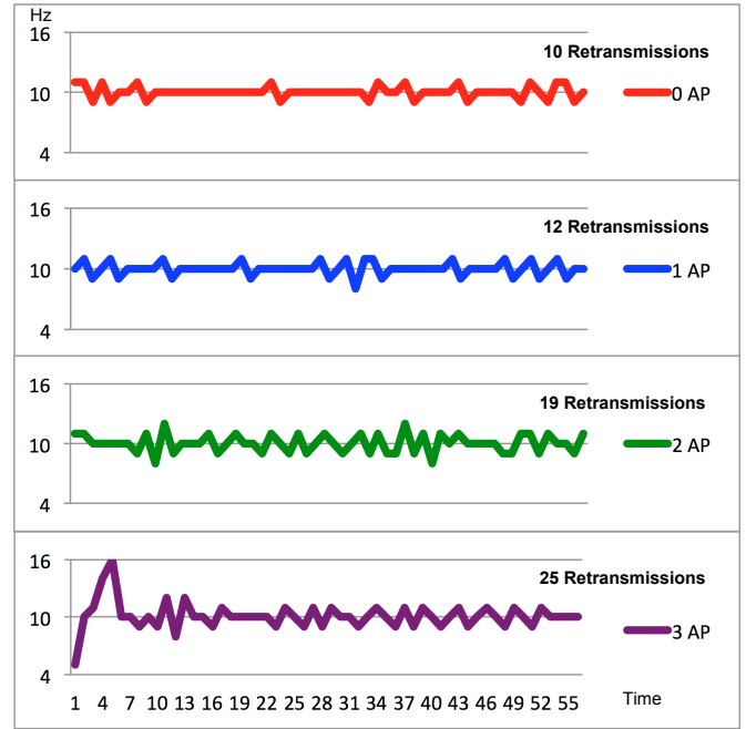
Fig. 3. Packet rate for different interference scenarios
