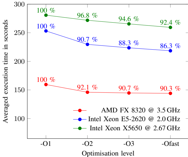
Fig. 1. Influence of compiler optimisation levels on execution time, averaged over 15 measurements for Data + Beacons configuration
