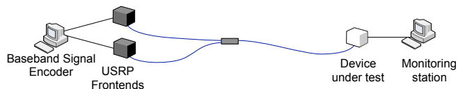
Fig. 3. Configuration used for measurement-based analysis of the capture effect. Two individually delayed IEEE802.11p frames are superimposed in radio frequency domain and fed to the receiver input of the DUT.
