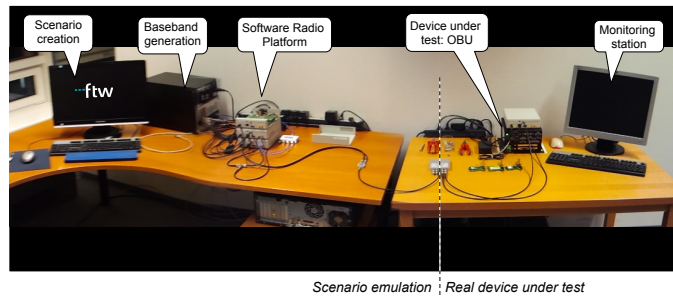
Fig. 2. Example configuration for testing an on-board unit (OBU)
