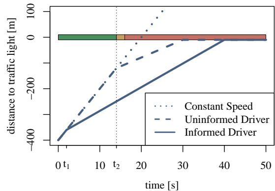
Figure 1. Trajectories of different scenarios at traffic lights where stopping can not be avoided
