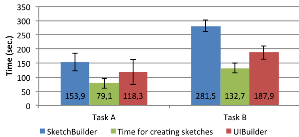
Figure 3. The diagram shows time for creating UIs with SketchBuilder and UIBuilder. Further, the time for creating UI sketches is depicted as separate series. It appears that drawing sketches takes a significant amount of time.
